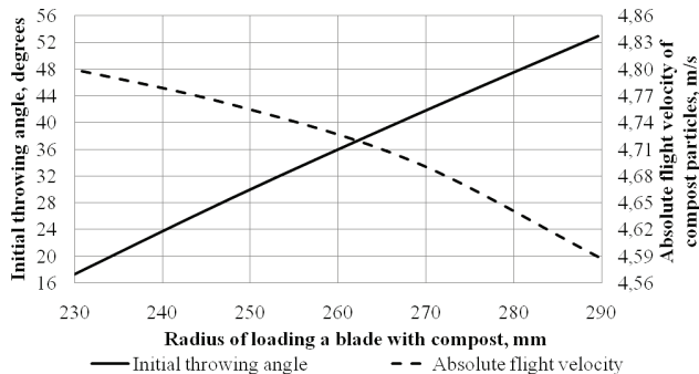
Fig. 7. Dependences of the initial throwing angle and absolute flight velocity of compost particles at increasing the radius of loading a blade with compost for the case when a compost particle is divided into four equal pieces
